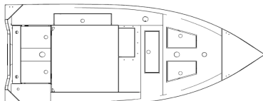
Bass Boat 430 | 450 | 480
