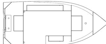
V fishing 370 | 390 | 435
